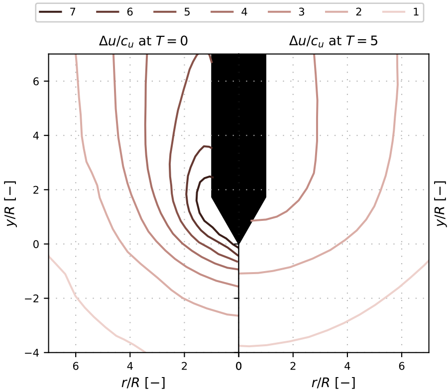
Figure 2.11: Excess pore pressure following undrained cone penetration at T = 0 (undrained) and after some dissipation at T = 5 , data from Teh and Houlsby (1991).
