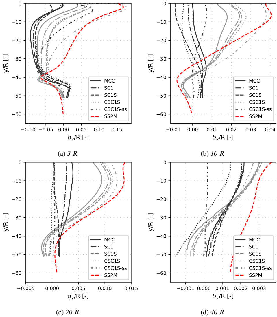
Figure 4.10: Vertical displacement from pile installation (light) and subsequent consolidation (dark) for four inclinometers (vertical cross sections) located at a radial distance of respectively 3R , 10R , 20R , and 40R . Influence of soft natural clay features indicated by including results from all constitutive models from Table 4.3.
