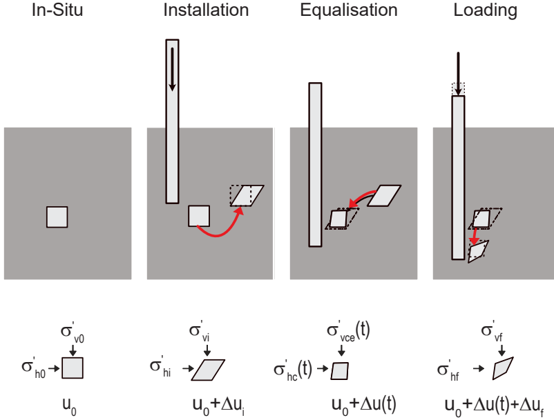
Figure 1.1: The pile cycle. Separation of the service life of a pile into four different stages. Adopted from Randolph and Gourvenec (2011).
