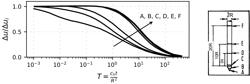
Figure 2.10: Dissipation at the pile shaft after undrained CPTu penetration at different vertical distances from the tip, from Teh and Houlsby (1991).
