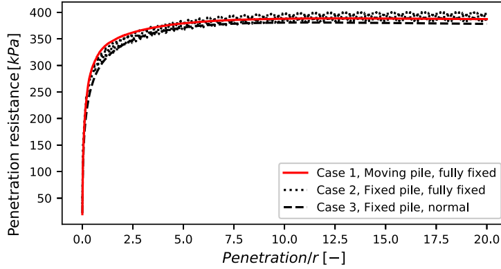
Figure 4.3: Cone tip resistance from simulations using the fixed pile method with two different ways of applying BC and the moving pile method. Results obtained using E/c_u = 150
