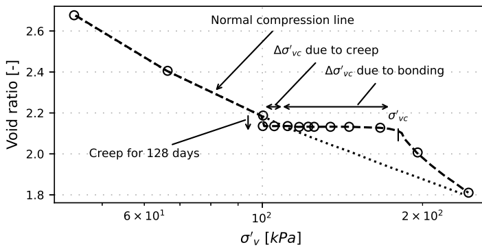
Figure 2.5: Influence of creep and bonding on the oedometric response of resedimented Jonqui re Clay, data from Leroueil (1996).
